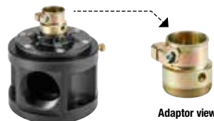
P/N 6199 Anodized aluminum pump base for nipple or suction tube G 2" (m)
